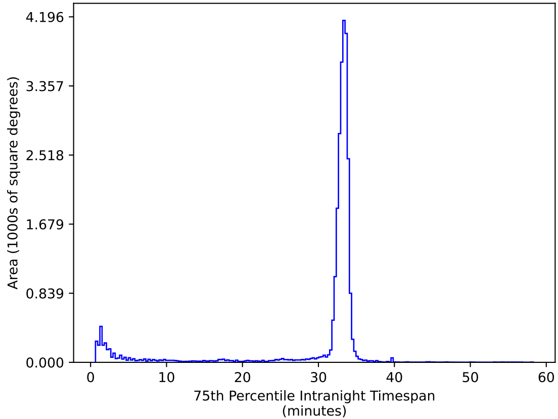
early_u_fpextra3.0_v3.4_10yrs All sky ug bands: 75th Percentile Intranight Timespan
