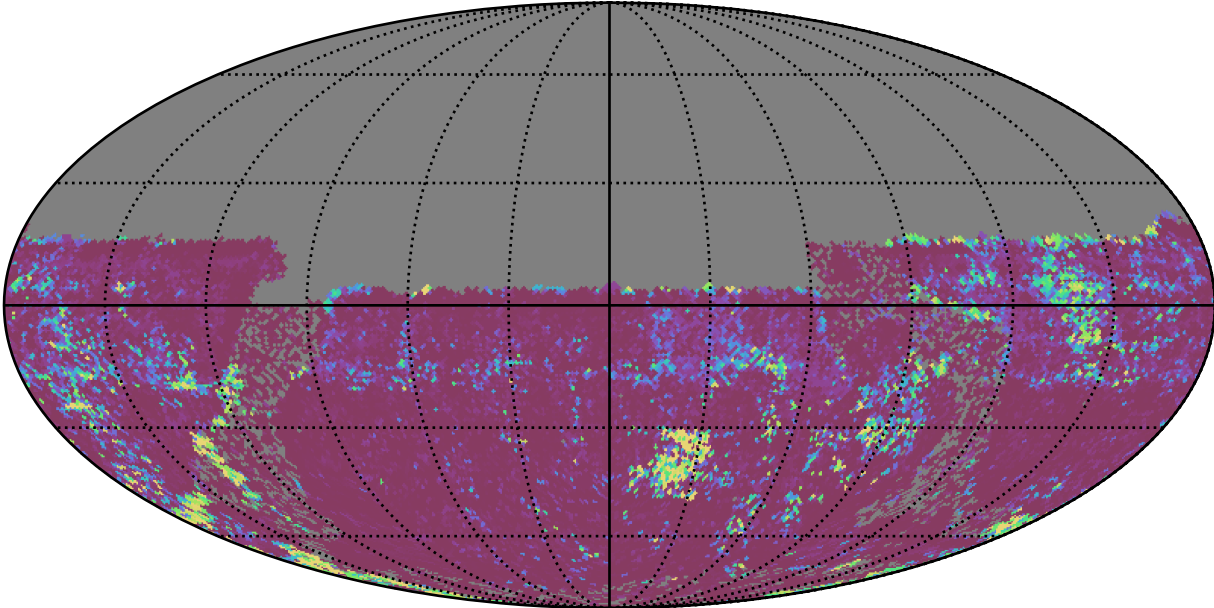
early_u_fpextra3.0_v3.4_10yrs All sky u band: 75th Percentile Intranight Timespan
