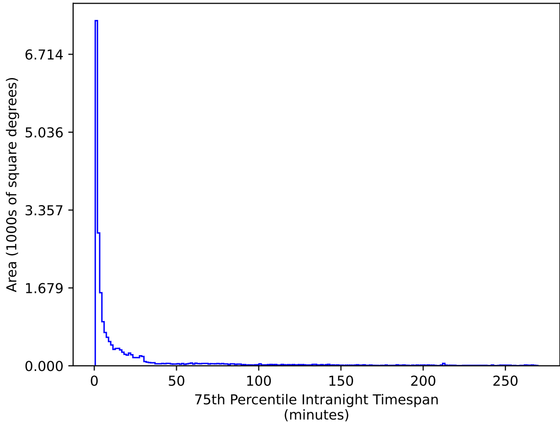
early_u_fpextra3.0_v3.4_10yrs All sky u band: 75th Percentile Intranight Timespan
