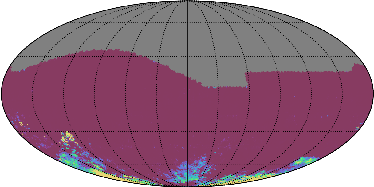
early_u_fpextra3.0_v3.4_10yrs All sky ri bands: 75th Percentile Intranight Timespan
