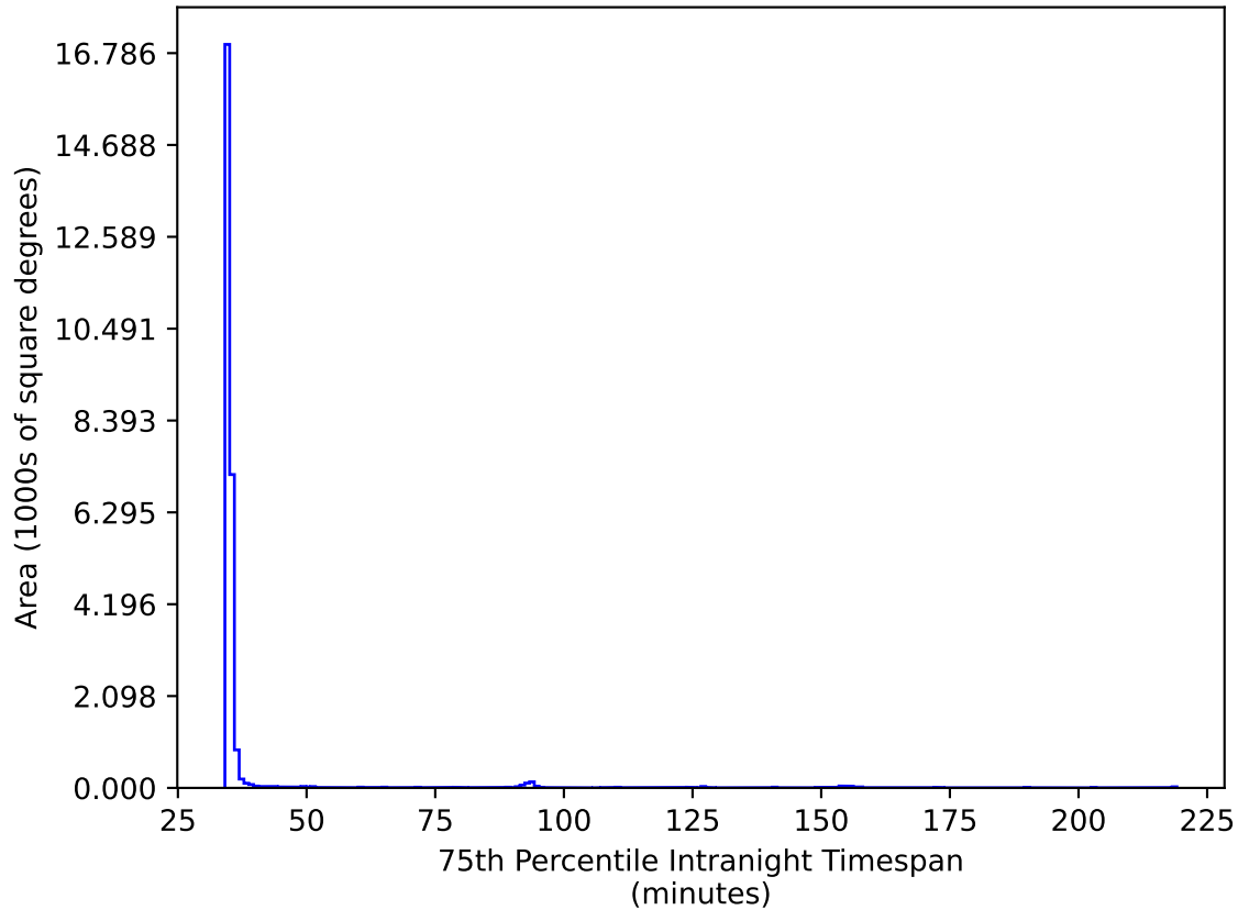
early_u_fpextra3.0_v3.4_10yrs All sky ri bands: 75th Percentile Intranight Timespan
