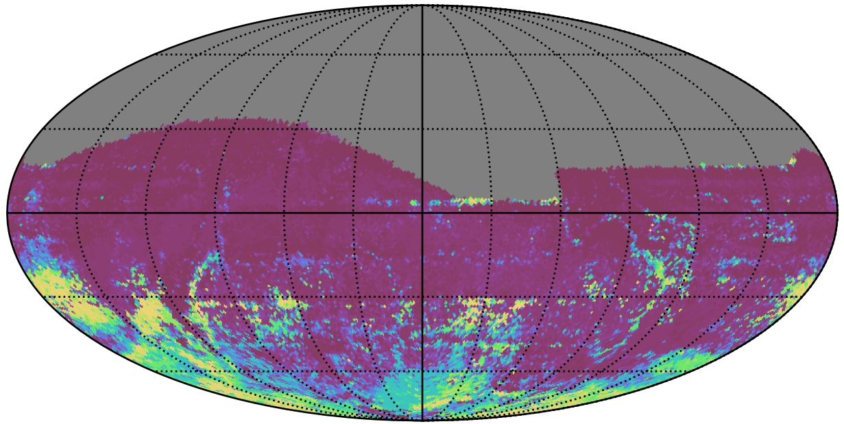
early_u_fpextra3.0_v3.4_10yrs All sky r band: 75th Percentile Intranight Timespan
