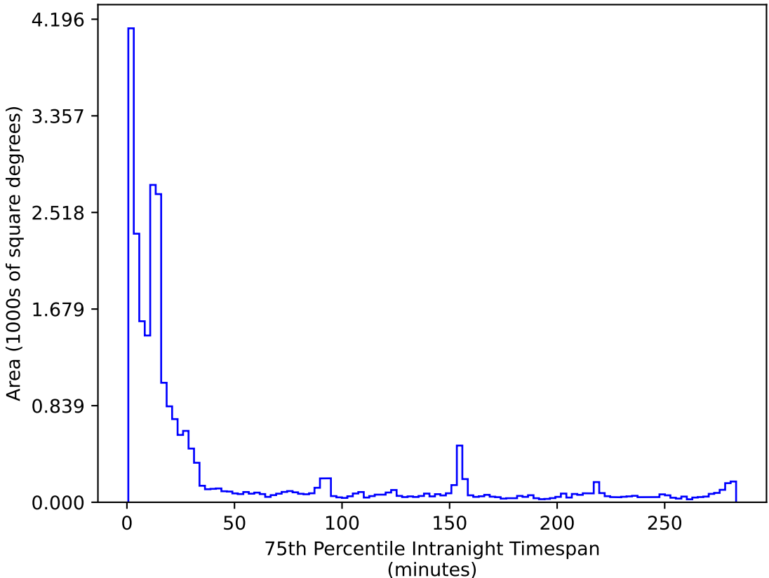
early_u_fpextra3.0_v3.4_10yrs All sky r band: 75th Percentile Intranight Timespan
