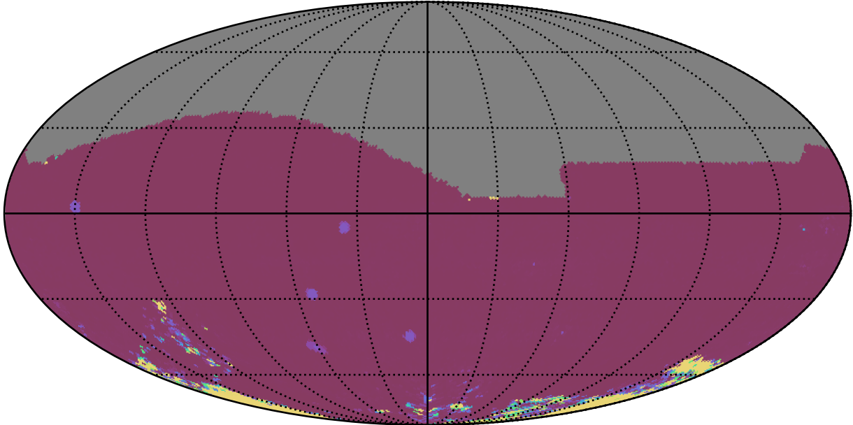
early_u_fpextra3.0_v3.4_10yrs All sky iz bands: 75th Percentile Intranight Timespan
