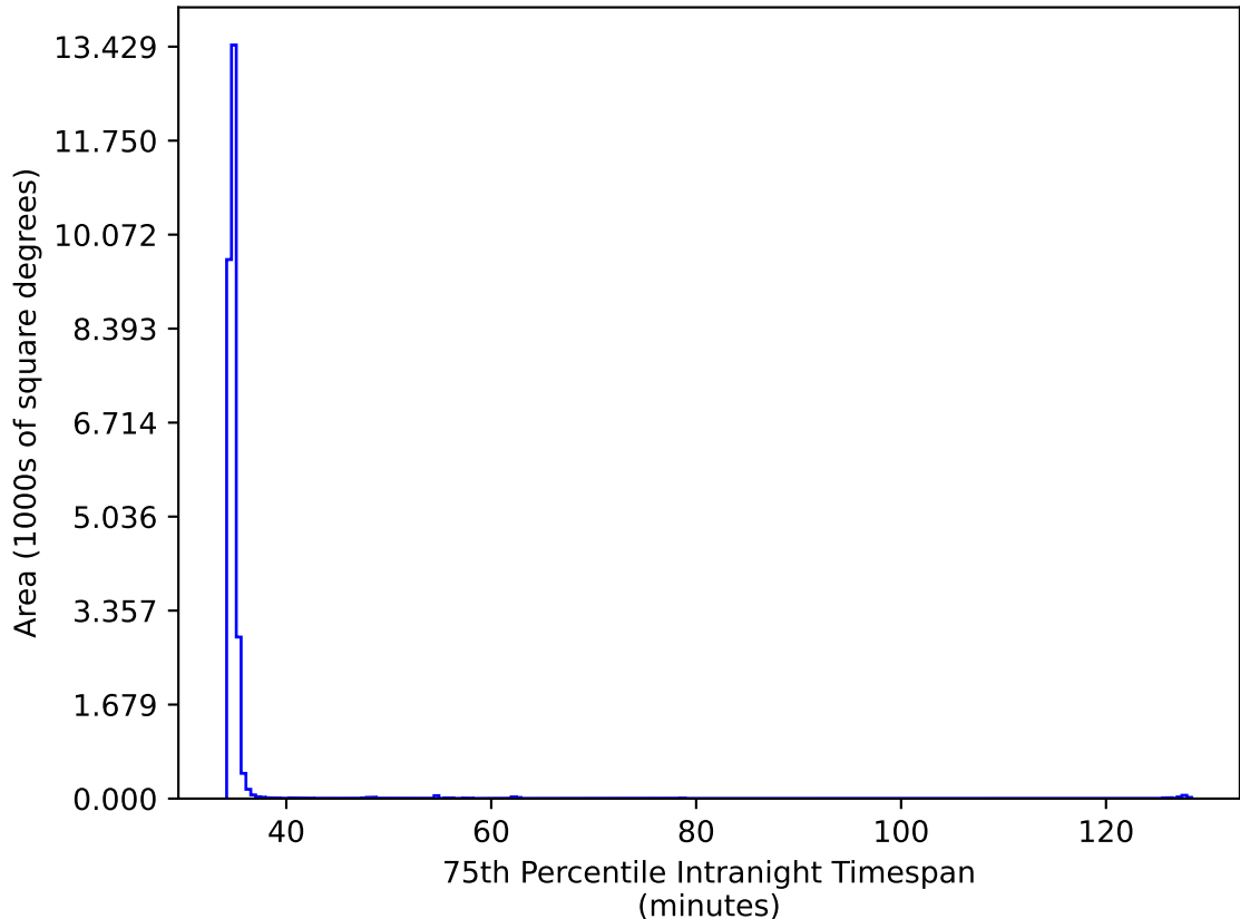
early_u_fpextra3.0_v3.4_10yrs All sky iz bands: 75th Percentile Intranight Timespan
