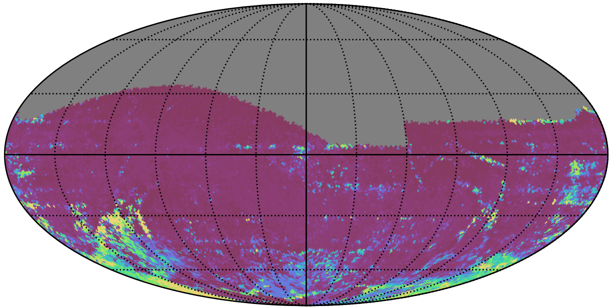
early_u_fpextra3.0_v3.4_10yrs All sky i band: 75th Percentile Intranight Timespan
