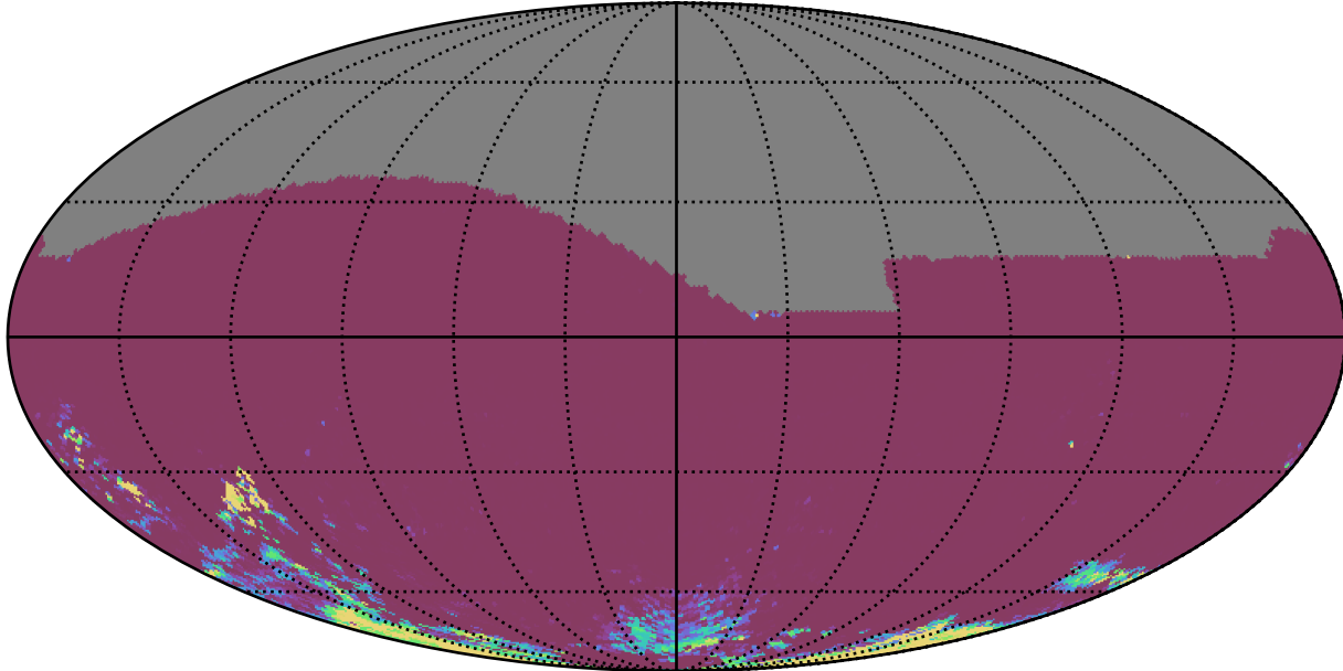
early_u_fpextra3.0_v3.4_10yrs All sky gr bands: 75th Percentile Intranight Timespan
