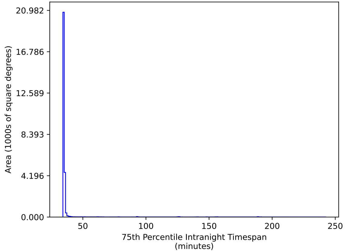
early_u_fpextra3.0_v3.4_10yrs All sky gr bands: 75th Percentile Intranight Timespan
