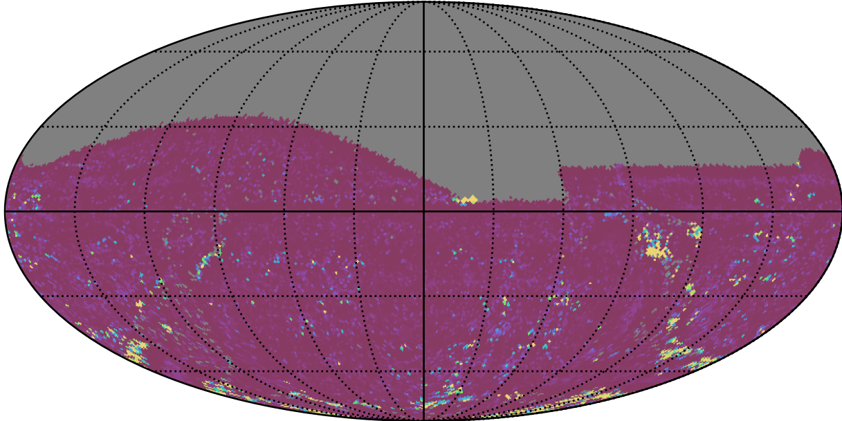
early_u_fpextra3.0_v3.4_10yrs All sky g band: 75th Percentile Intranight Timespan
