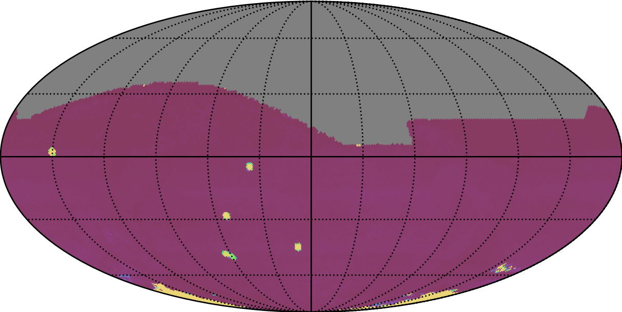
early_u_fpextra3.0_v3.4_10yrs All sky all bands: 75th Percentile Intranight Timespan
