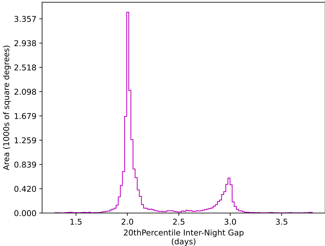
early_u_fpextra3.0_v3.4_10yrs WFD z band: 20thPercentile Inter-Night Gap
