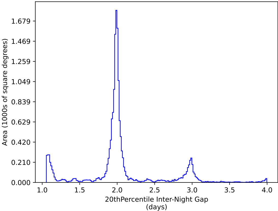
early_u_fpextra3.0_v3.4_10yrs WFD y band: 20thPercentile Inter-Night Gap
