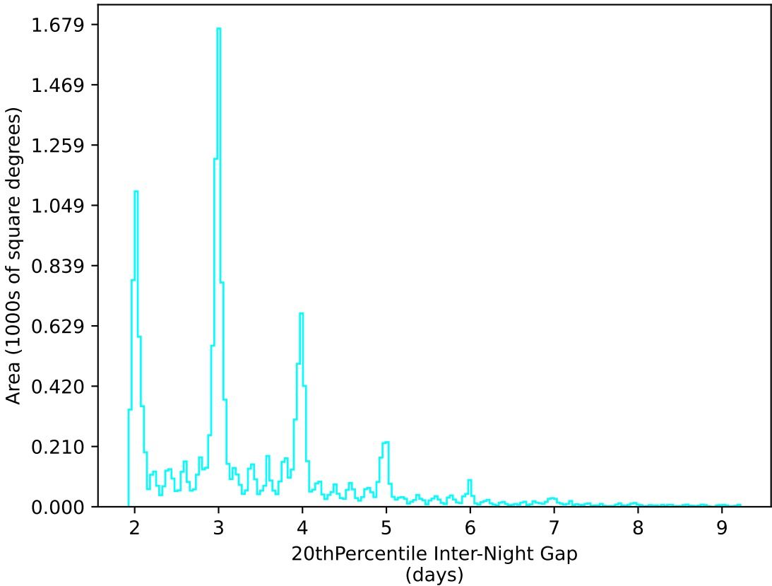
early_u_fpextra3.0_v3.4_10yrs WFD u band: 20thPercentile Inter-Night Gap
