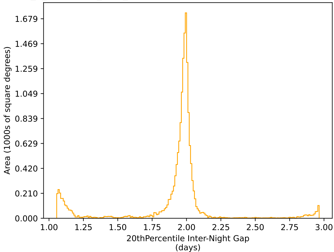
early_u_fpextra3.0_v3.4_10yrs WFD r band: 20thPercentile Inter-Night Gap
