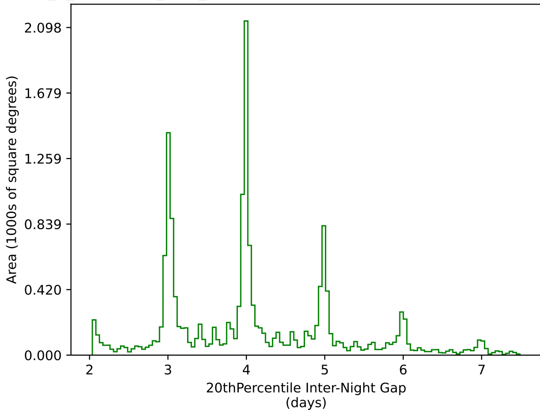
early_u_fpextra3.0_v3.4_10yrs WFD g band: 20thPercentile Inter-Night Gap
