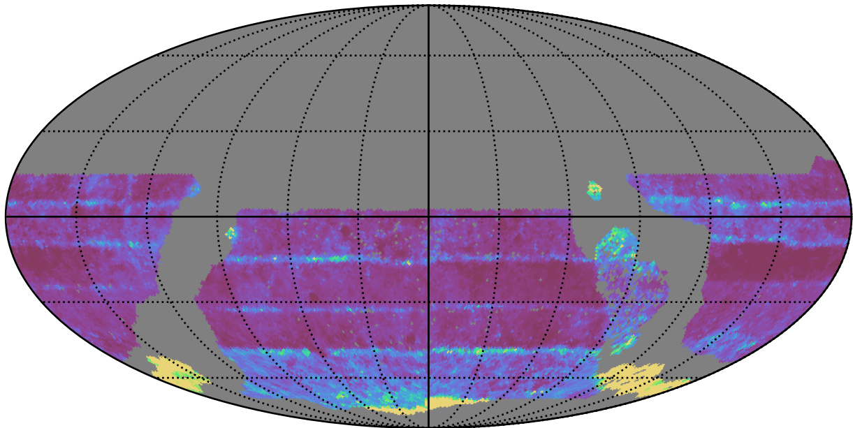
early_u_fpextra3.0_v3.4_10yrs WFD all bands: 20thPercentile Inter-Night Gap
