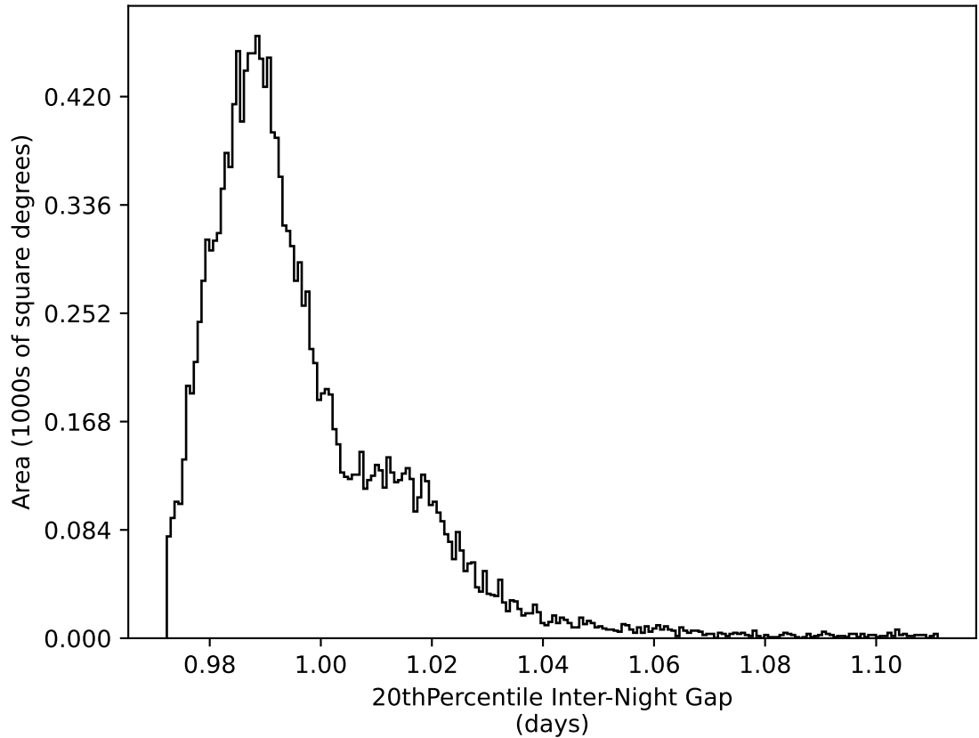
early_u_fpextra3.0_v3.4_10yrs WFD all bands: 20thPercentile Inter-Night Gap
