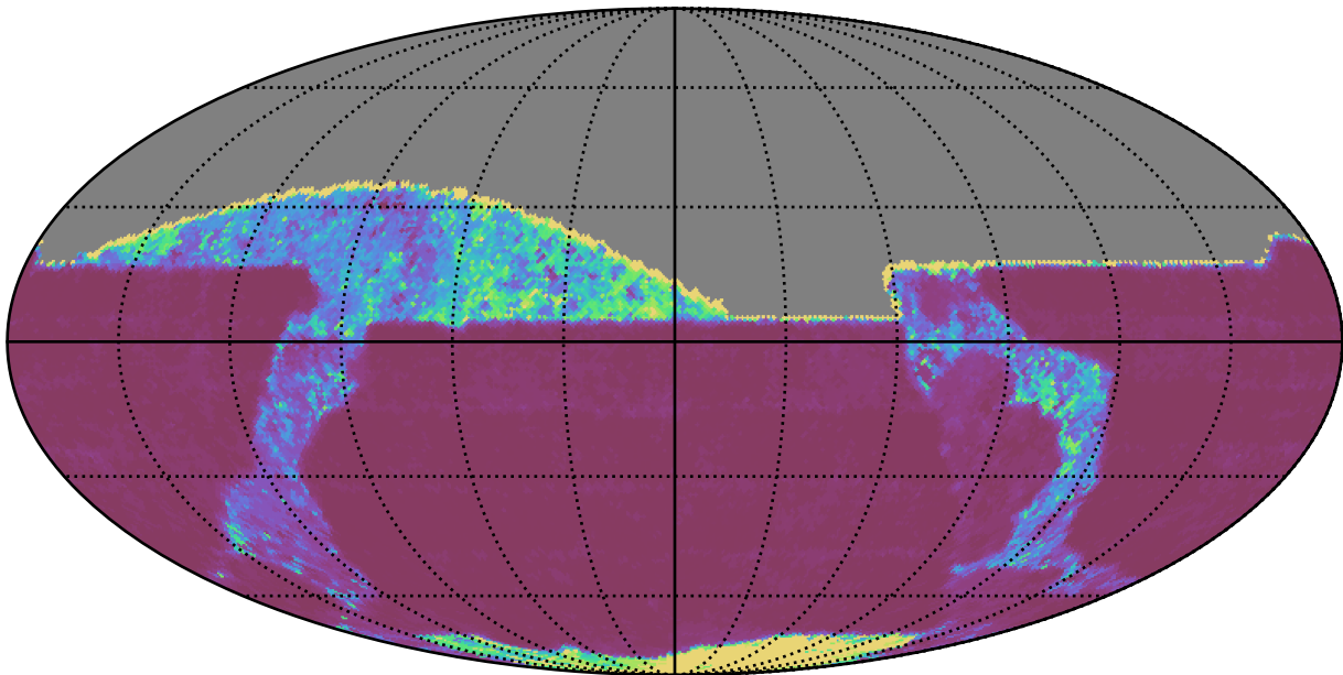
early_u_fpextra3.0_v3.4_10yrs All sky z band: 20thPercentile Inter-Night Gap
