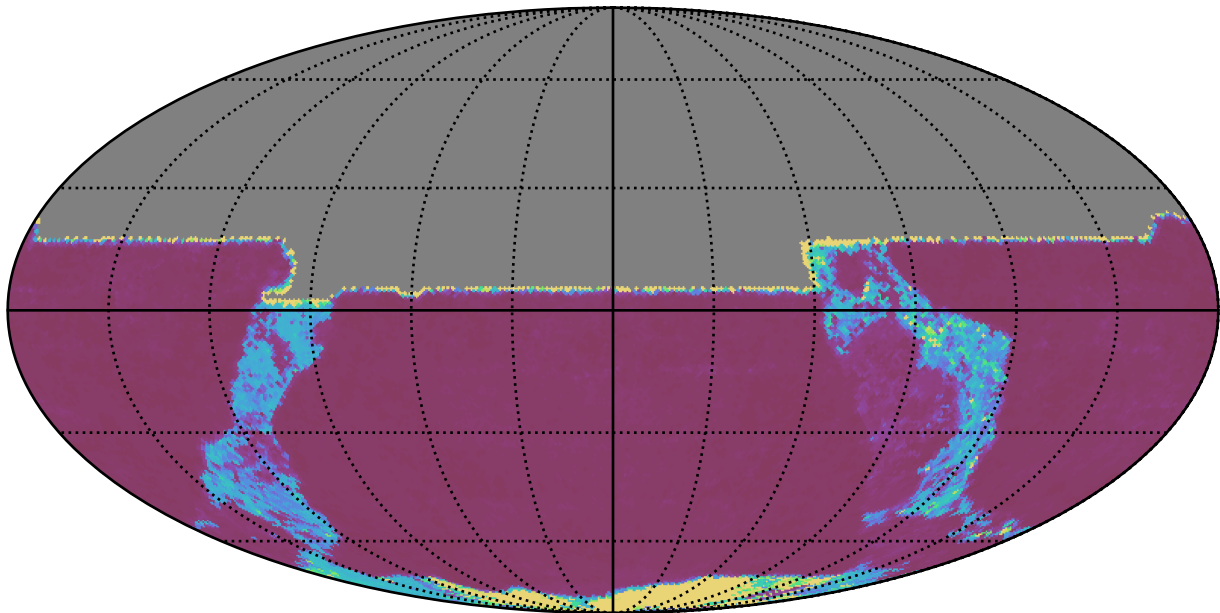
early_u_fpextra3.0_v3.4_10yrs All sky y band: 20thPercentile Inter-Night Gap
