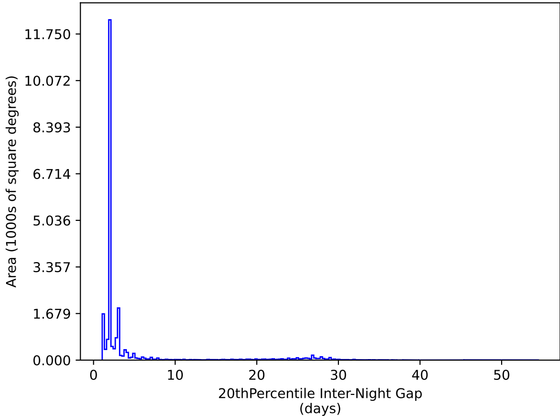
early_u_fpextra3.0_v3.4_10yrs All sky y band: 20thPercentile Inter-Night Gap
