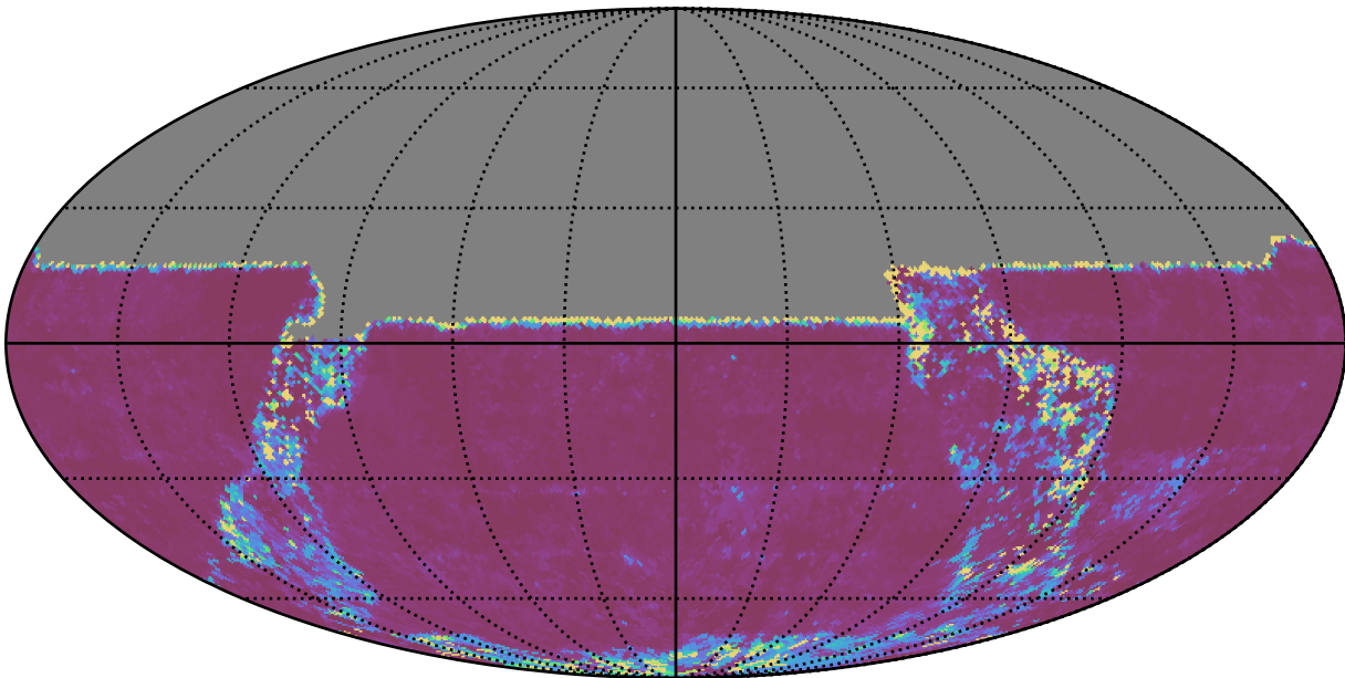
early_u_fpextra3.0_v3.4_10yrs All sky u band: 20thPercentile Inter-Night Gap
