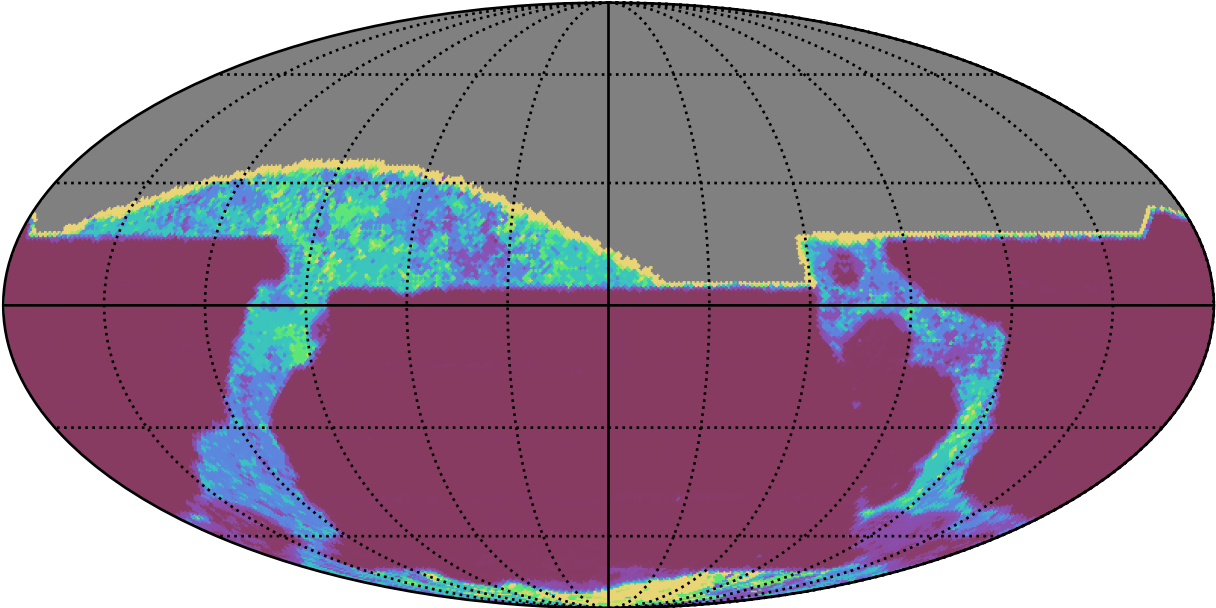
early_u_fpextra3.0_v3.4_10yrs All sky all bands: 20thPercentile Inter-Night Gap
