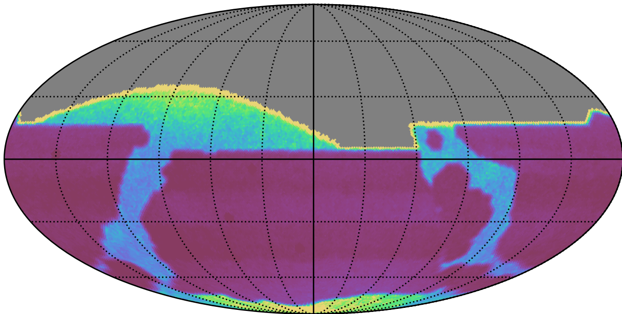
early_u_fpextra3.0_v3.4_10yrs : properMotion
