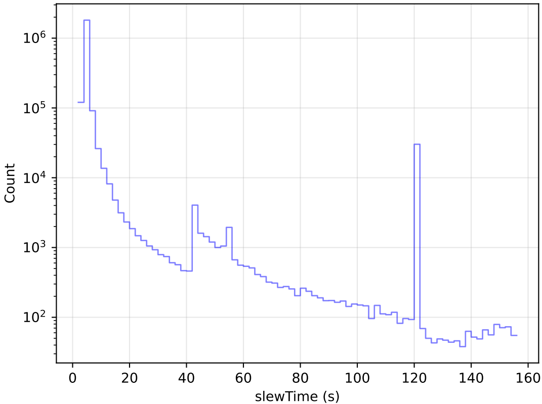
early_u_fpextra3.0_v3.4_10yrs All visits: Slew Time Histogram
