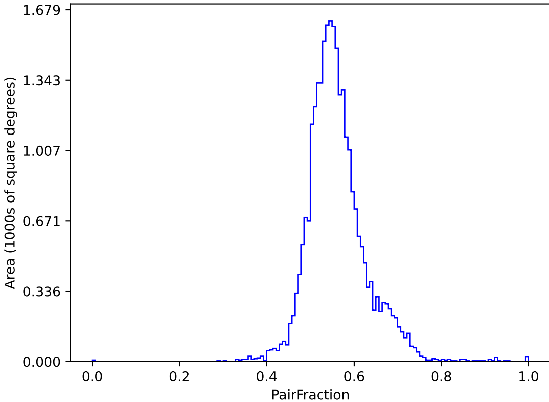
early_u_fpextra3.0_v3.4_10yrs (g or r or i): PairFraction
