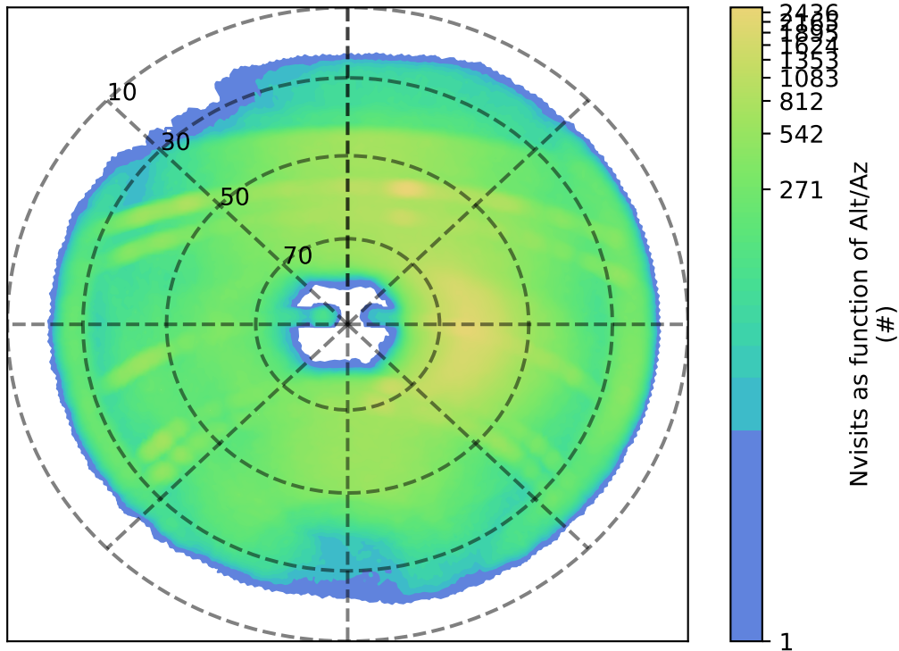
early_u_fpextra3.0_v3.4_10yrs z: Nvisits as function of Alt/Az
