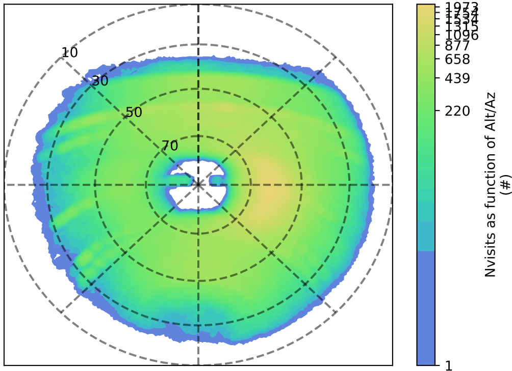
early_u_fpextra3.0_v3.4_10yrs y: Nvisits as function of Alt/Az
