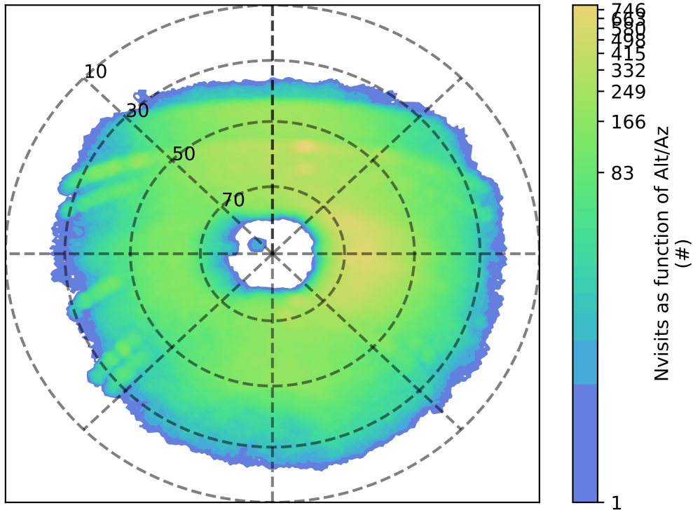
early_u_fpextra3.0_v3.4_10yrs u: Nvisits as function of Alt/Az
