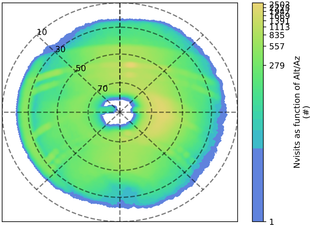
early_u_fpextra3.0_v3.4_10yrs r: Nvisits as function of Alt/Az
