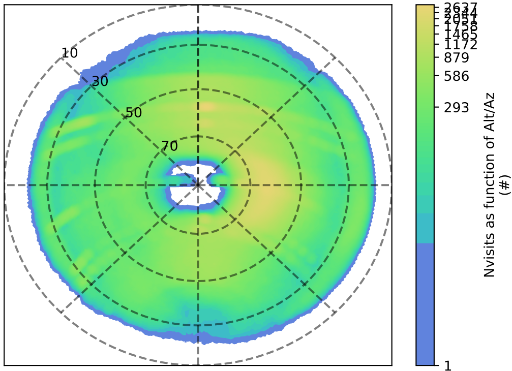
early_u_fpextra3.0_v3.4_10yrs i: Nvisits as function of Alt/Az
