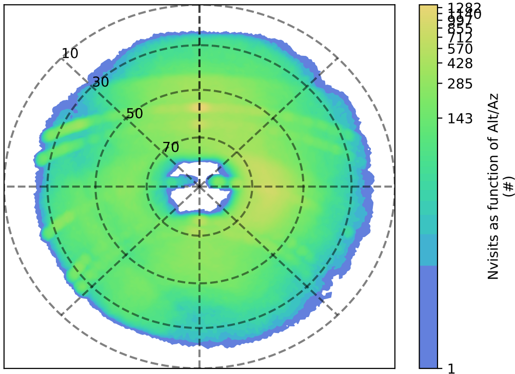
early_u_fpextra3.0_v3.4_10yrs g: Nvisits as function of Alt/Az
