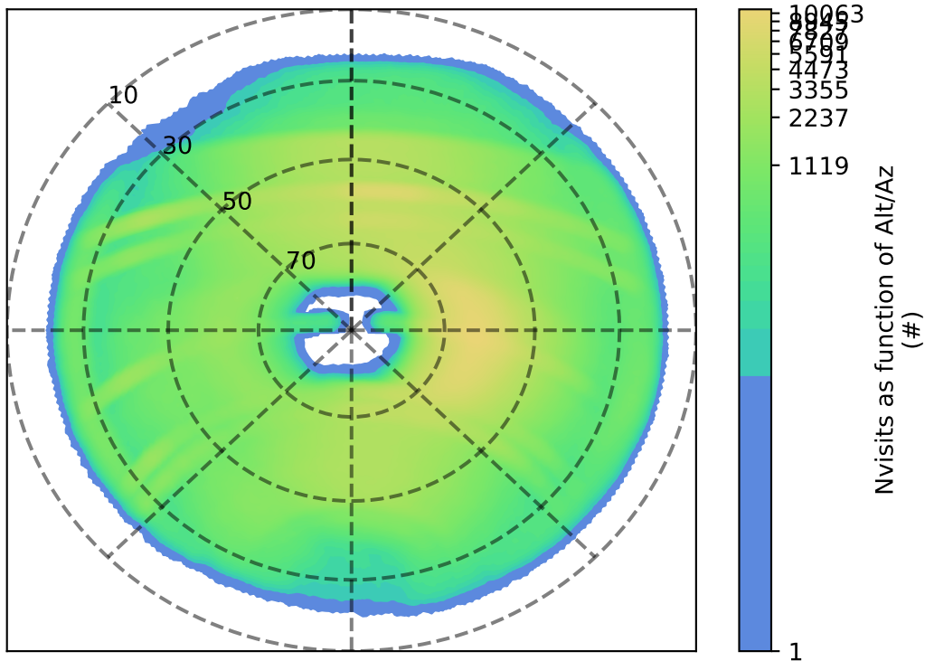
early_u_fpextra3.0_v3.4_10yrs : Nvisits as function of Alt/Az
