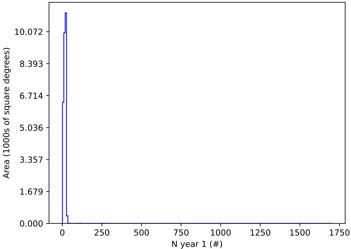
early_u_fpextra3.0_v3.4_10yrs r and night < 365: N year 1
