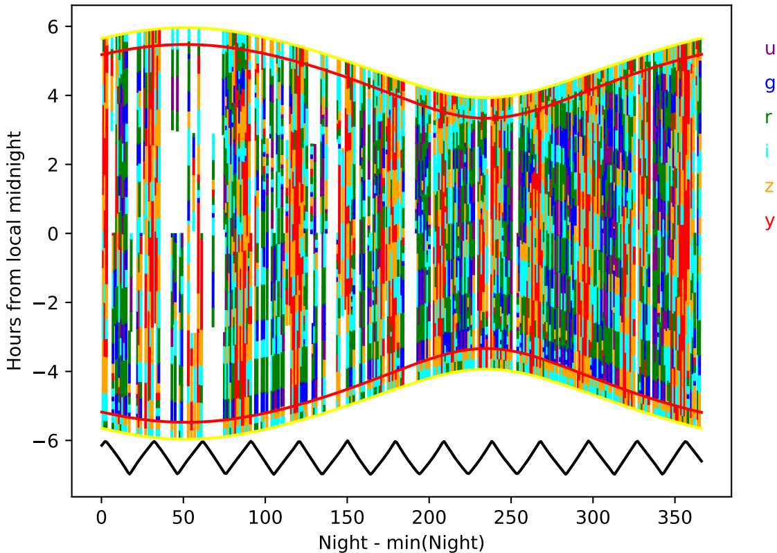
early_u_fpextra3.0_v3.4_10yrs year 9-10: Hourglass
