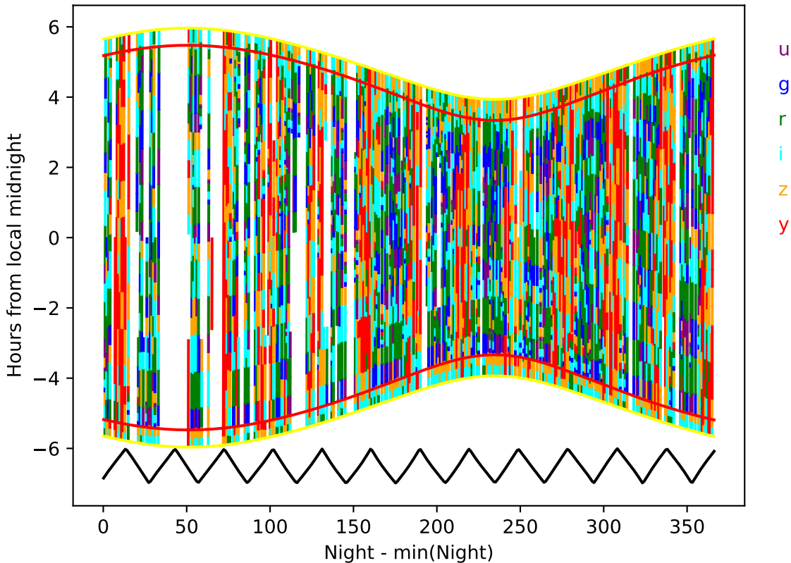
early_u_fpextra3.0_v3.4_10yrs year 8-9: Hourglass
