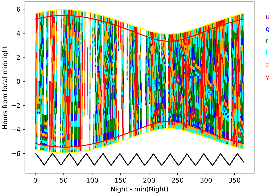
early_u_fpextra3.0_v3.4_10yrs year 1-2: Hourglass
