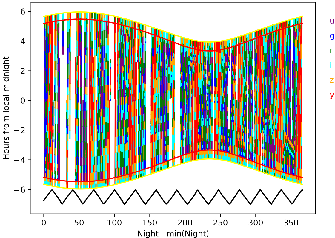
early_u_fpextra3.0_v3.4_10yrs year 0-1: Hourglass
