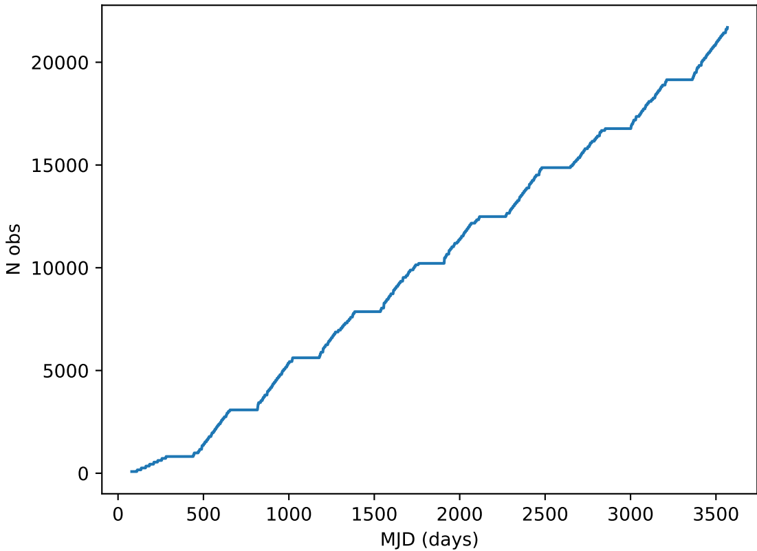
early_u_fpextra3.0_v3.4_10yrs note like DD:XMM_LSS%: Cumulative
