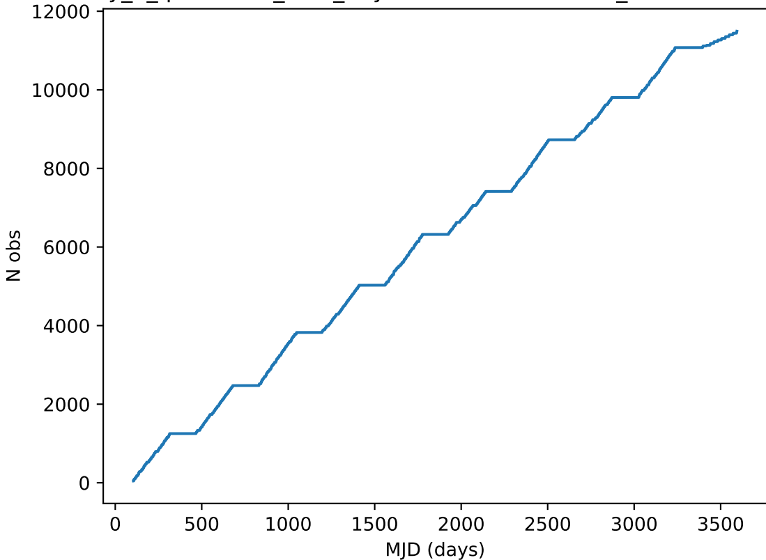
early_u_fpextra3.0_v3.4_10yrs note like DD:EDFS_b%: Cumulative
