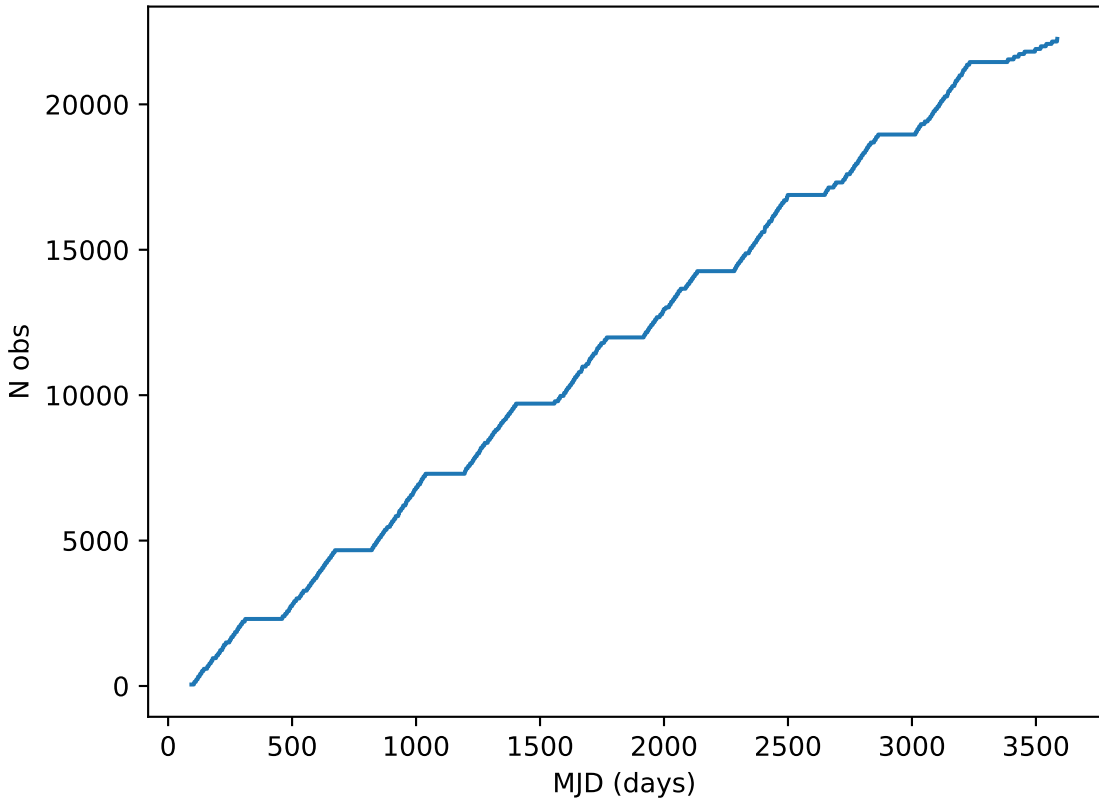
early_u_fpextra3.0_v3.4_10yrs note like DD:ECDFS%: Cumulative
