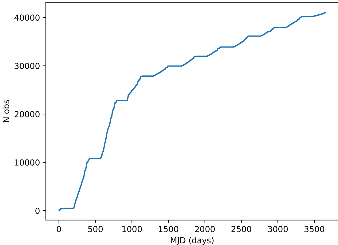
early_u_fpextra3.0_v3.4_10yrs note like DD:COSMOS%: Cumulative
