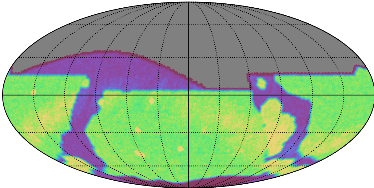
early_u_fpextra3.0_v3.4_10yrs r: Count observationStartMJD
