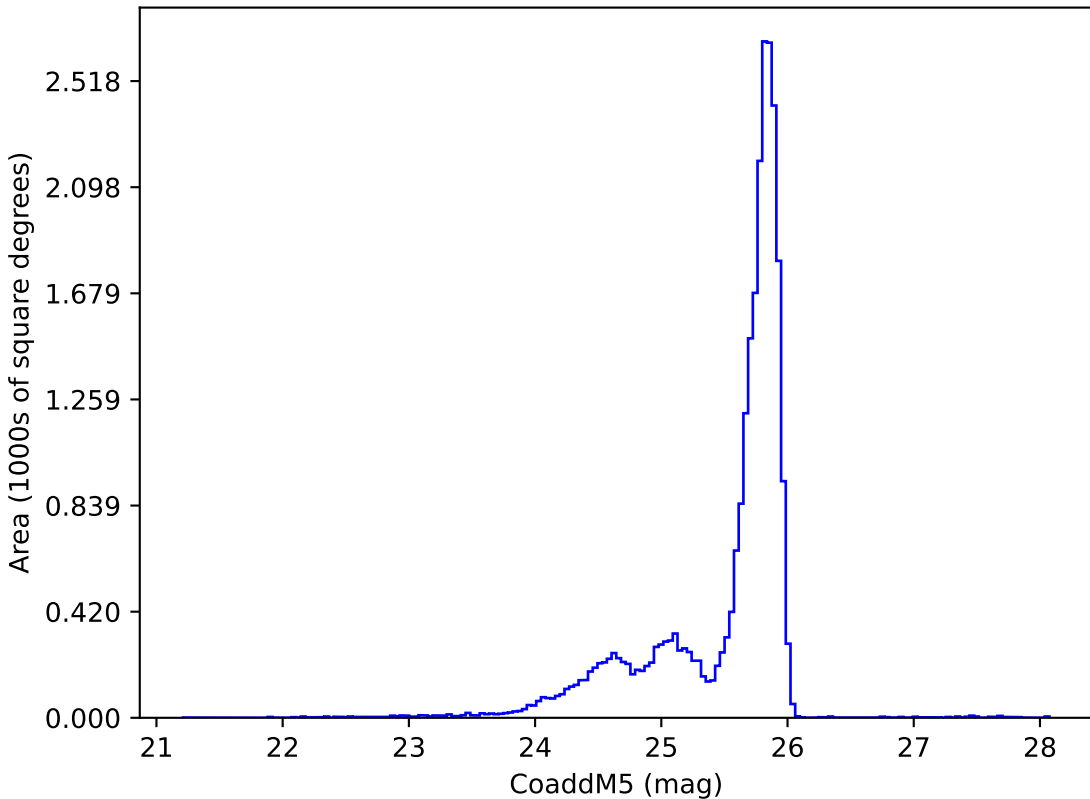
early_u_fpextra3.0_v3.4_10yrs z: CoaddM5
