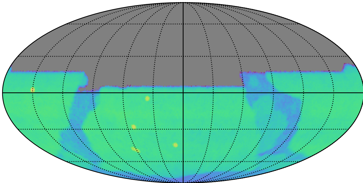
early_u_fpextra3.0_v3.4_10yrs u: CoaddM5
