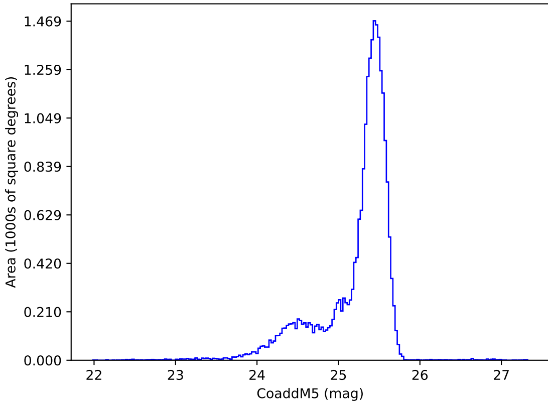
early_u_fpextra3.0_v3.4_10yrs u: CoaddM5
