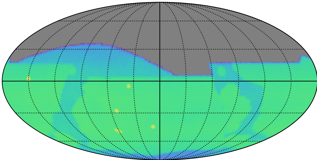
early_u_fpextra3.0_v3.4_10yrs r: CoaddM5
